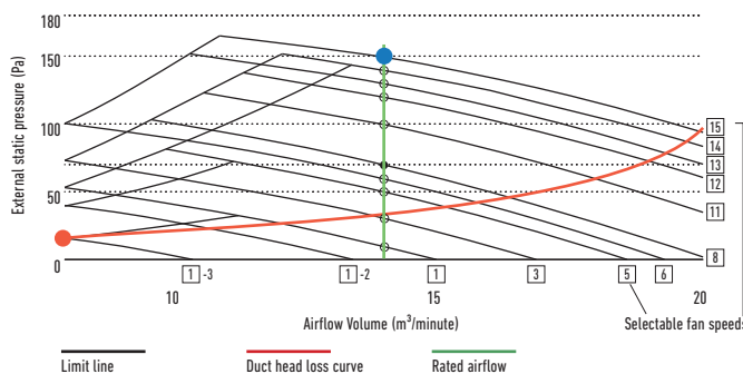
Diagram 1 S-22MF2E5A
