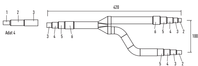
Liquid tubing
