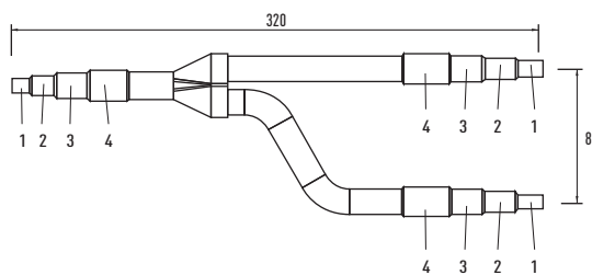
Liquid tubing
