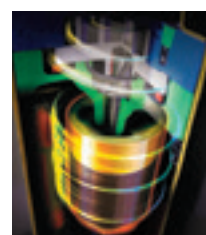
Panasonic twin Rotary Compressor. A large capacity inverter compressor has been adopted. This new compressor features wider and 0,1Hz step inverter control.
